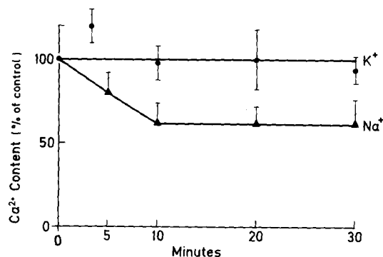
Fig. 4. Influence of K^+ and Na^+ on efflux of ^{45}Ca^{2+} from vesicles preloaded with the isotope. Secretory vesicles were incubated at 30^\circ C for 15 min in 0.5 mM EGTA, 20 mM Tes (pH 7.3), 10^{-4} M free Ca^{2+} with tracer, 260 mM sucrose and 20 mM KCl. They were then transferred to media containing 130 mM KCl or NaCl with the sucrose concentration reduced to give an osmolality of approx. 315 mosmol/kg.
