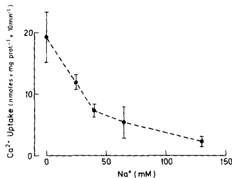
Fig. 3. Inhibition of ^{45}\text{Ca}^{2+} uptake by increasing concentration of \text{Na}^+ in the incubation medium. Secretory vesicles were incubated at 30^\circ\text{C} for 10 min in the presence of 10^{-4}\text{ M} free \text{Ca}^{2+} , 0.5 mM EGTA, 20 mM Tes (pH 7.3), increasing concentration of \text{Na}^+ and decreasing concentration of sucrose (total osmolarity of medium about 315 mosmol/kg) as described in Methods.
