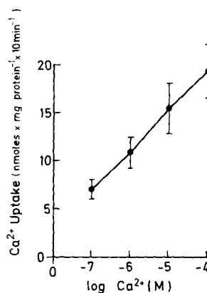
Fig. 2. Ca 2+ uptake at various concentrations of free Ca 2+ . Secretory vesicles were incubated at various concentrations of free Ca 2+ in a medium containing 20 mM KCl, 260 mM sucrose, 0.5 mM EGTA, 20 mM Tes (pH 7.3) at 30°C for 10 min. Protein concentration was 50 \mu\text{g} in a total volume of 200 \mu\text{l} . The calcium concentrations were calculated and controlled by a calcium ion specific electrode, as described in Methods. (5 expts., bars indicate S.D.)
