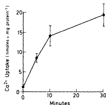
Fig. 1. Time dependence of Ca 2+ uptake into purified secretory vesicles from ox neurohypophyses. Secretory vesicles were incubated in the presence of 10^{-4} M free Ca 2+ in 20 mM KCl, 260 mM sucrose, 0.5 mM EGTA, 20 mM Tes (pH 7.3) at 30°C as described in Methods. Filtration and washing of the samples were complete within 30 s. Protein concentration was 50 \mu\text{g} in a volume of 200 \mu\text{l} . (5 expts., bars indicate S.D.)
