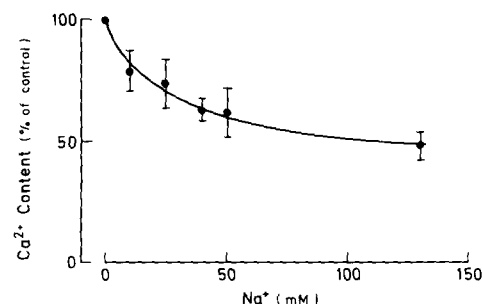
Fig. 5. Na^+ stimulation of efflux by Na^+ in increasing concentrations. Experimental conditions as in Fig. 4.
